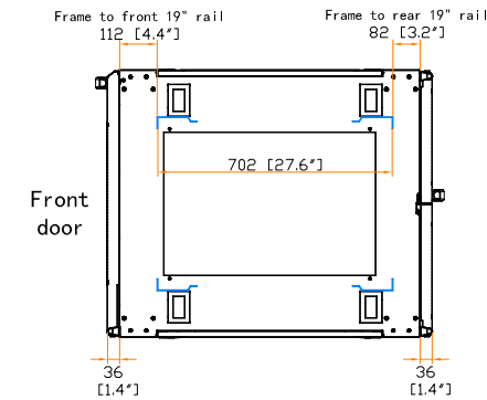
19" rail position
