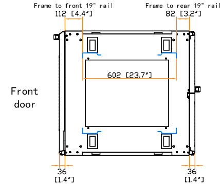
19" rail position
