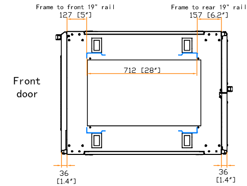
19" rail position
