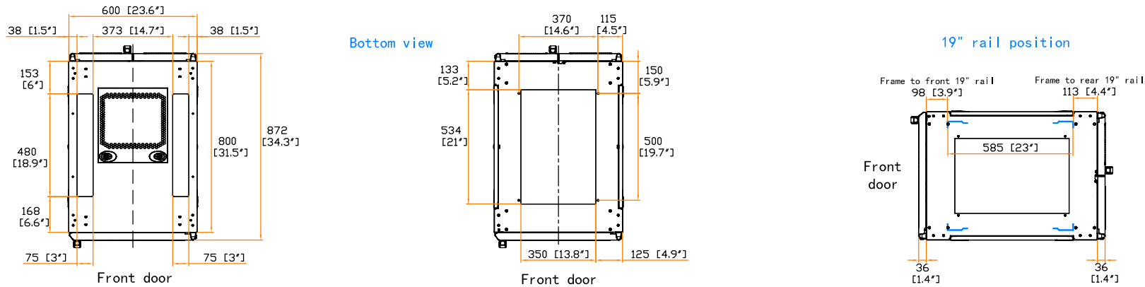
Top view
