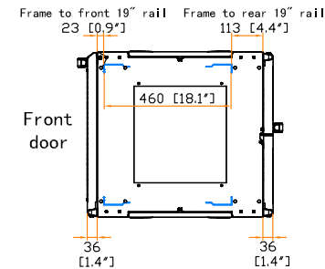
19" rail position
